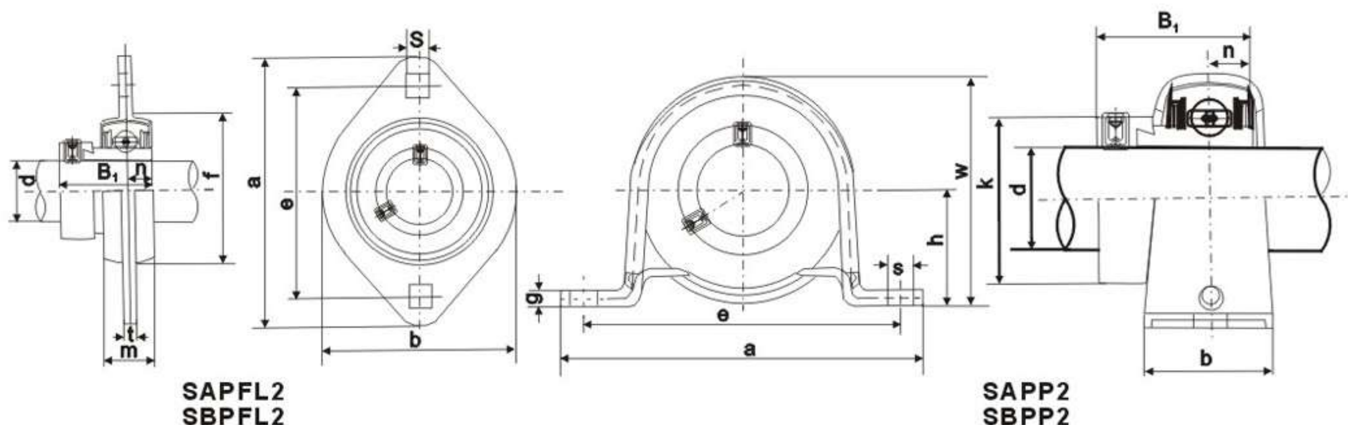
Pressed Housing (light-duty)
