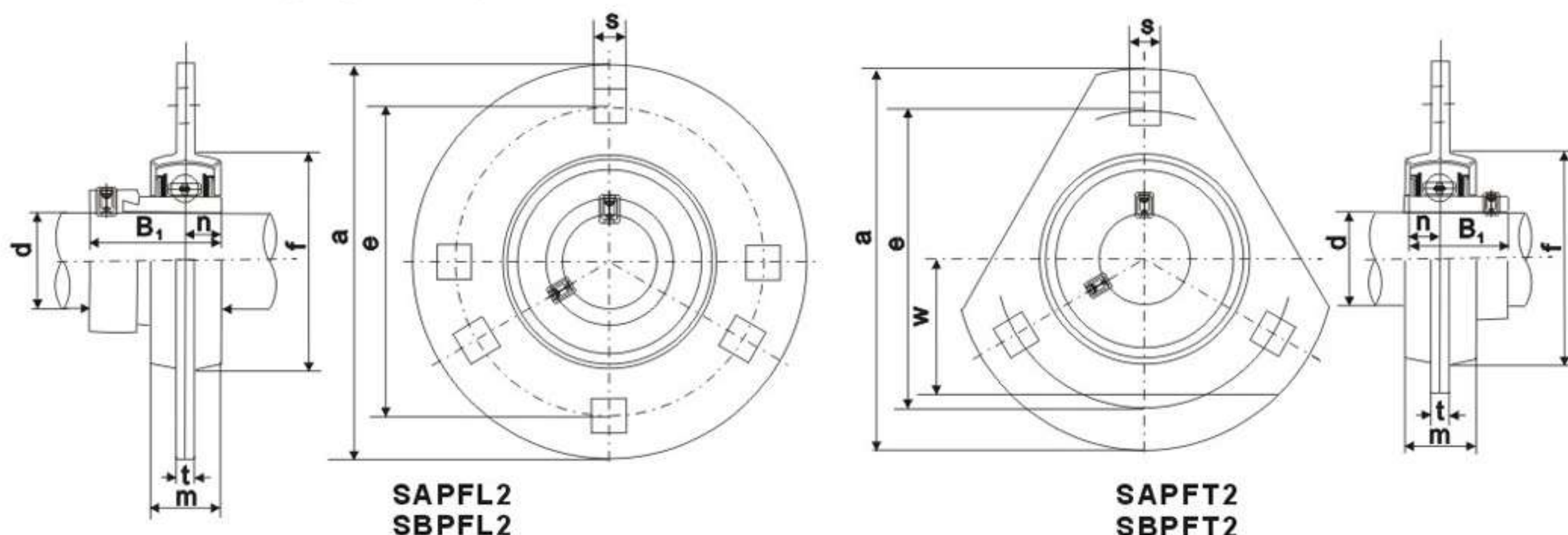
Pressed Housing (light-duty)
